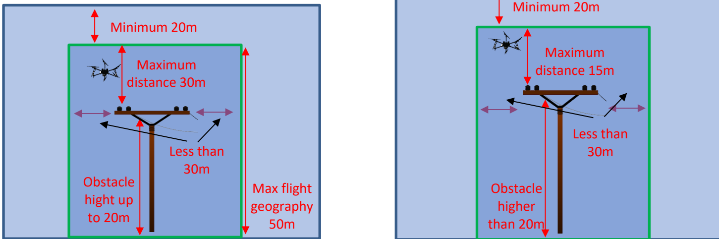
Figure 1 — Flight geography and operational volume when the operation is not conducted in reserved or segregated area
